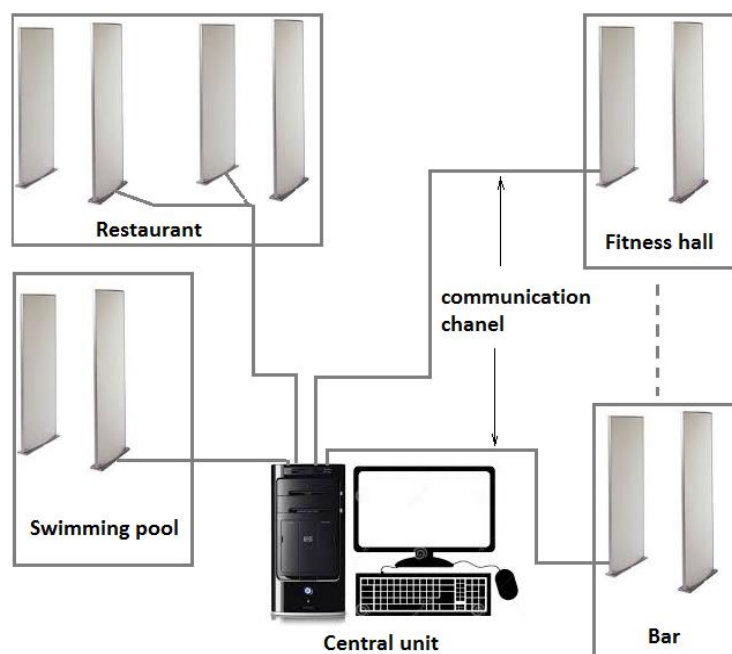
Figure 2 – Tracking system infrastructure
